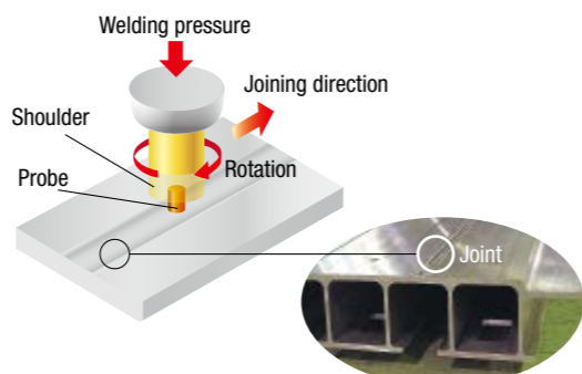
Friction Stir Welding (FSW) technology for high strength joints
